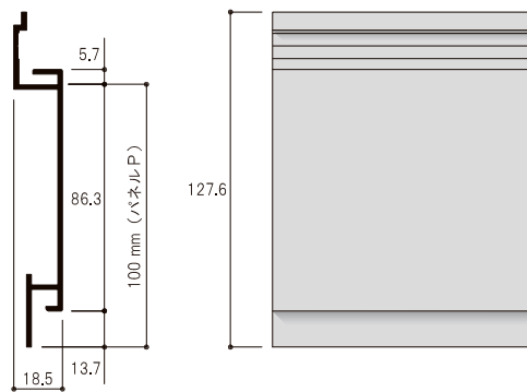
HP 100P 2730 W
